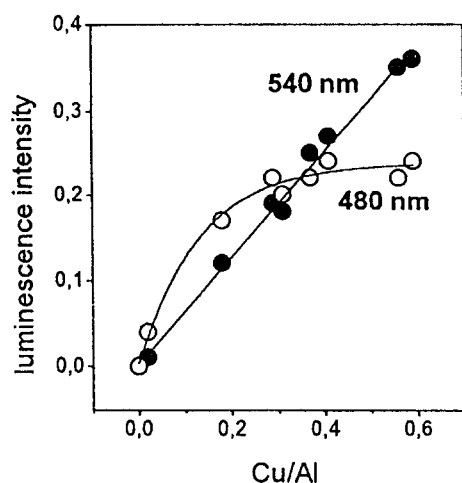
Fig. 3. Dependence of the \text{Cu}^+ luminescence intensity of individual bands on the Cu loading of ZSM-5.
